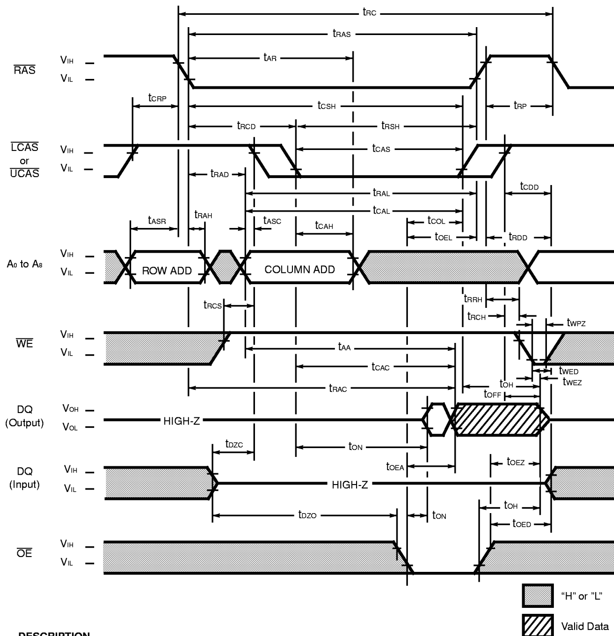
Fig. 5 – READ CYCLE
