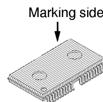
Plastic TSOP Package (FPT-44P-M07) (Normal Bend)
