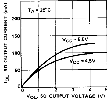
Fig. 31 – SD OUTPUT CURRENT vs SD OUTPUT VOLTAGE
