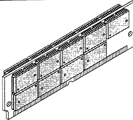
72-PAD PLASTIC SINGLE IN-LINE TYPE MODULE (CASE No.: MSS-72P-P31)
