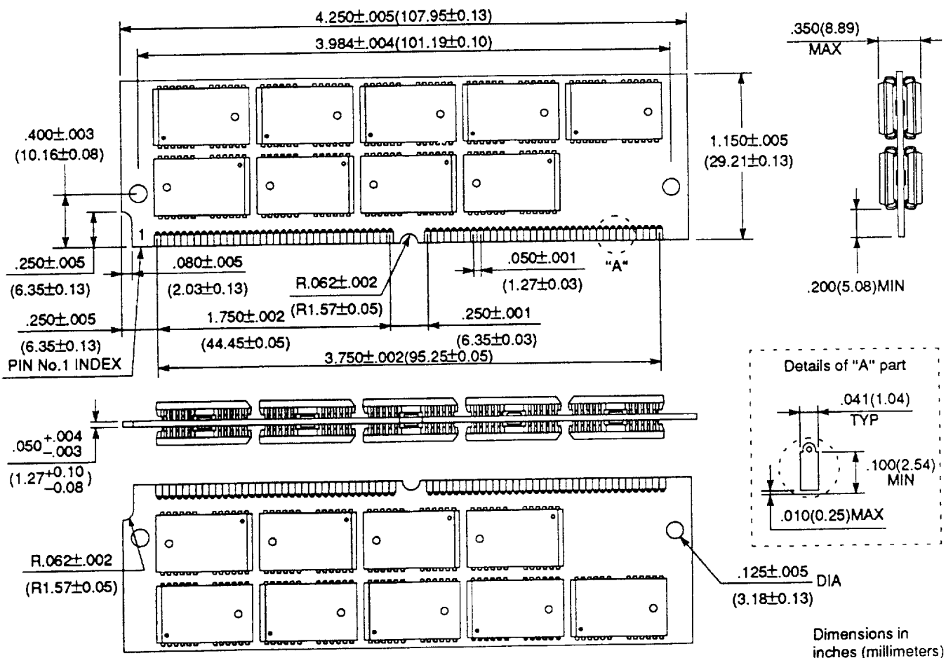
72-PAD PLASTIC SINGLE IN-LINE TYPE MODULE (CASE No.: MSS-72P-P31)
