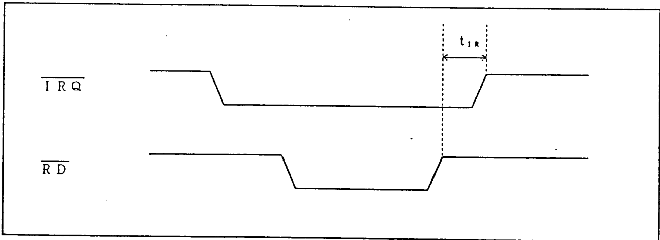
Figure 5.2 \overline{IRQ} timing
