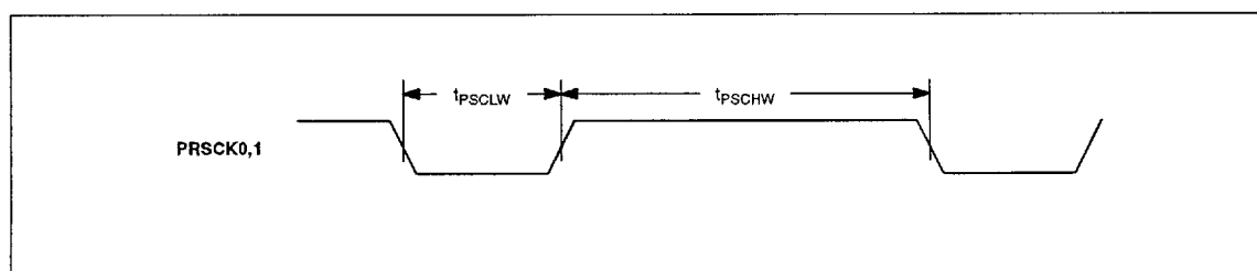
Figure 46. Prescaler Output Clock Timing Diagram
