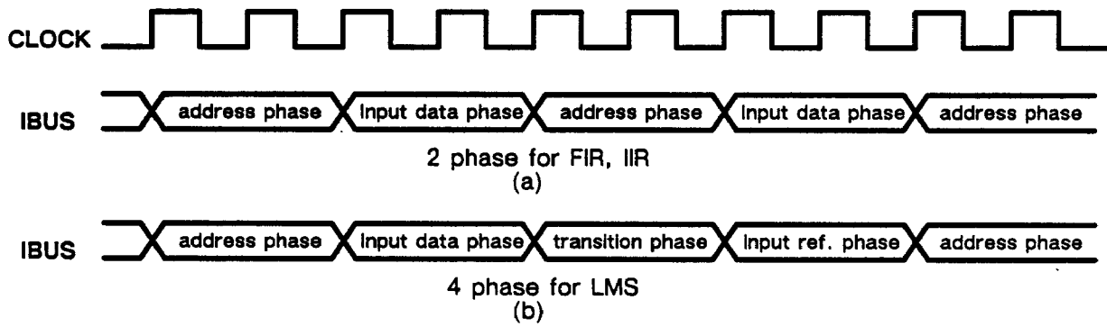
FIGURE 8 IBUS PROTOCOL
