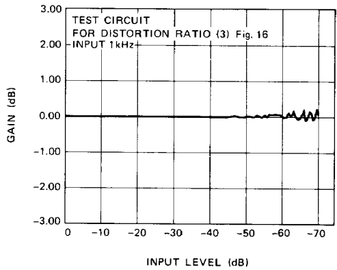
Fig. 29 – INPUT LEVEL vs. GAIN
