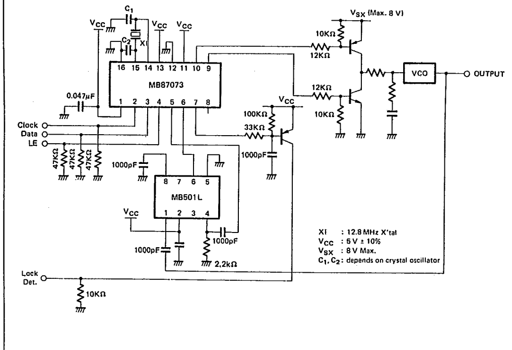
Fig. 3 — TYPICAL APPLICATION EXAMPLE
