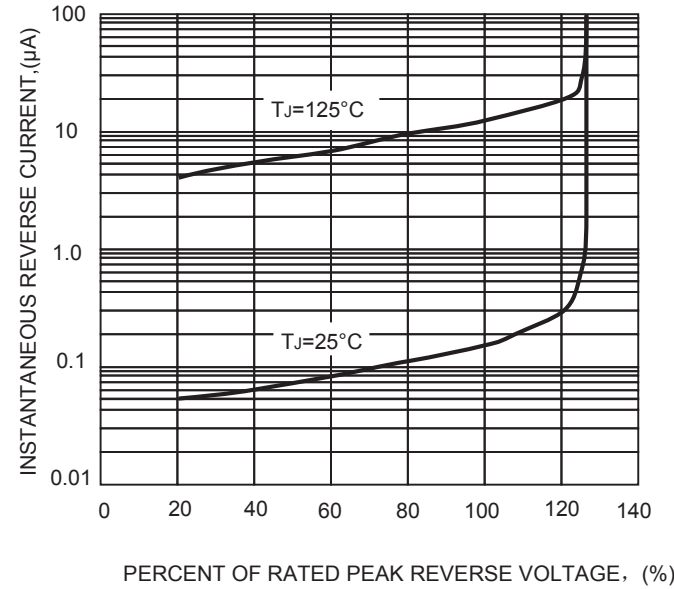
FIG.3-TYPICAL REVERSE CHARACTERISTICS
