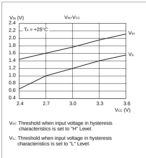
(4) "H" Level Input Voltage/"L" Level Input Voltage (Hysteresis Input)
