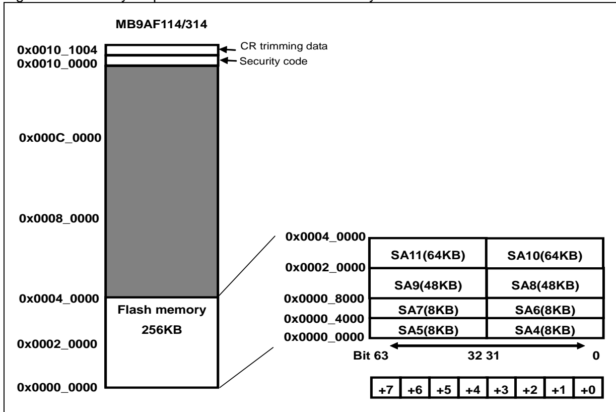
Figure 2-3 Memory map of MB9AF114/314 flash memory
