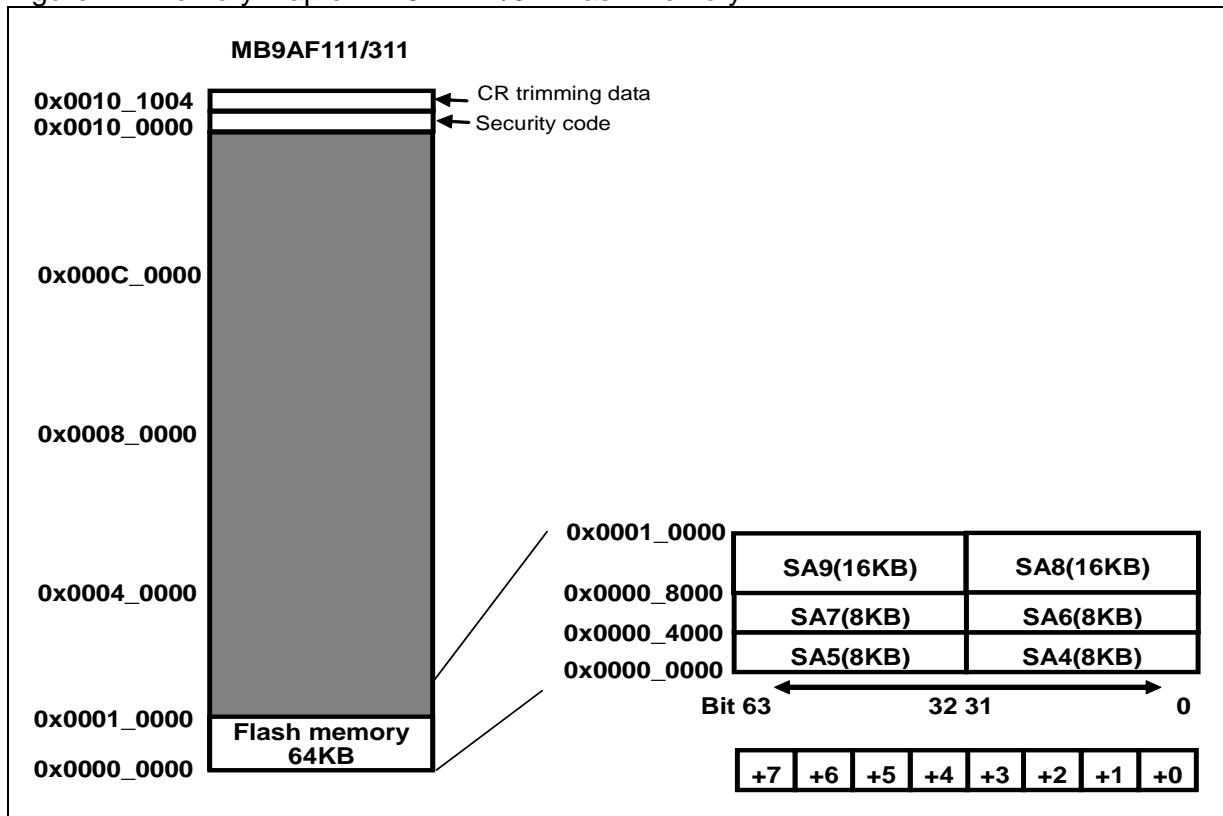
Figure 2-1 Memory map of MB9AF111/311 flash memory
