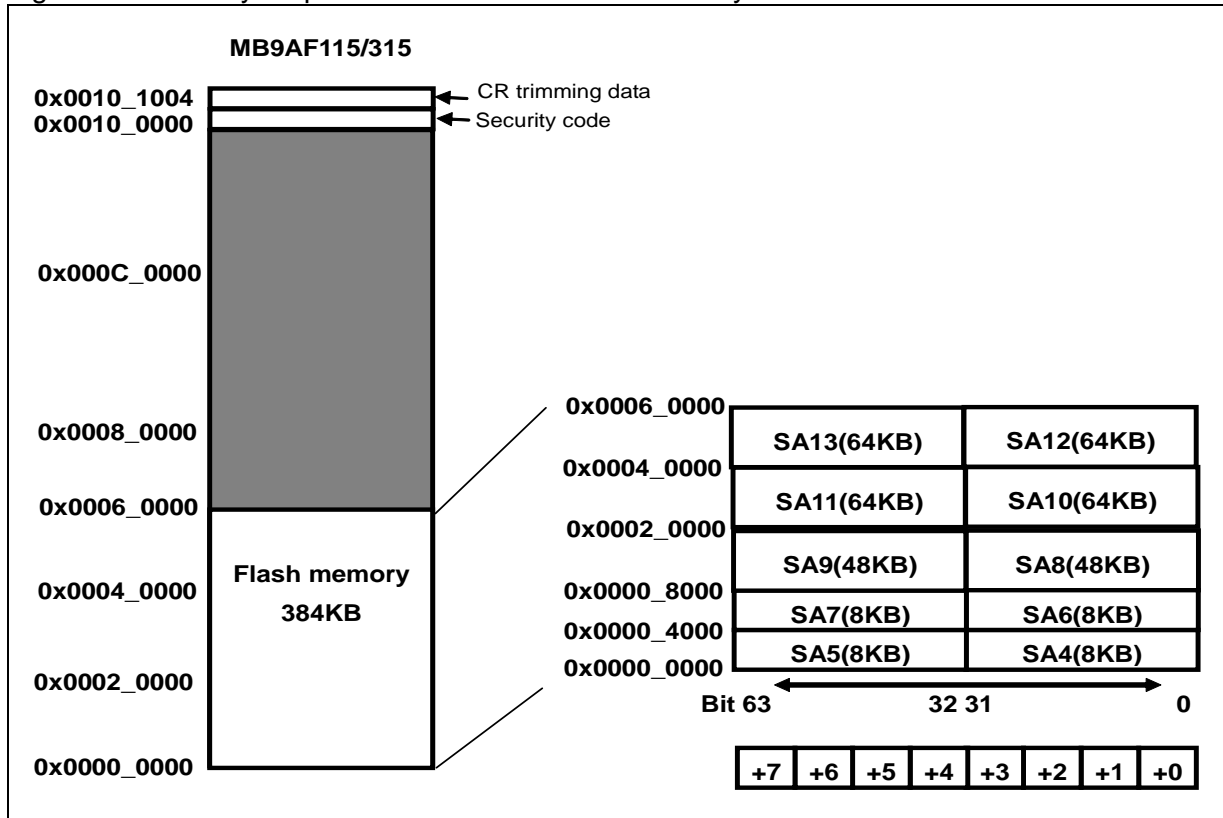
Figure 2-4 Memory map of MB9AF115/315 flash memory
