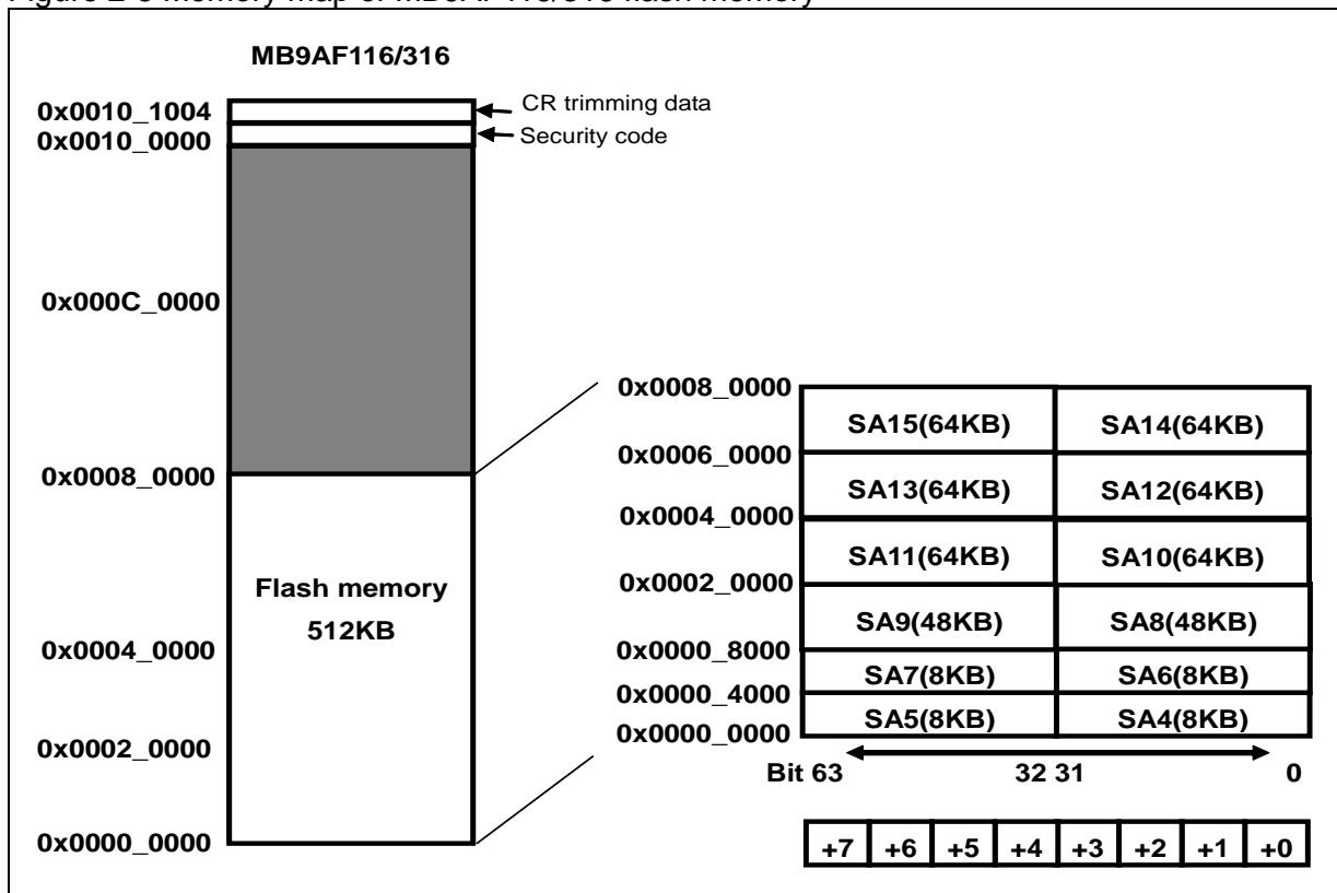
Figure 2-5 Memory map of MB9AF116/316 flash memory
