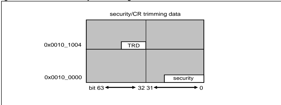
Figure 2-6 Address of security/CR trimming data
