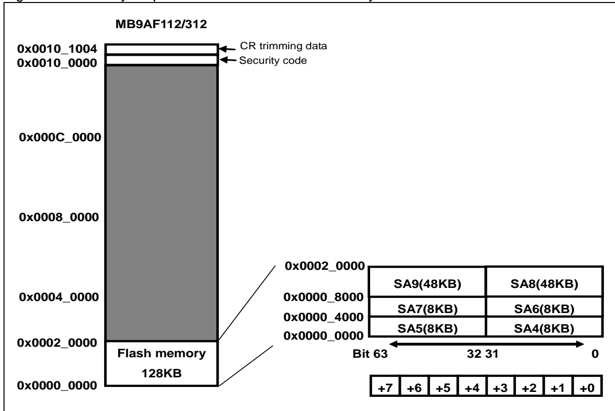
Figure 2-2 Memory map of MB9AF112/312 flash memory
