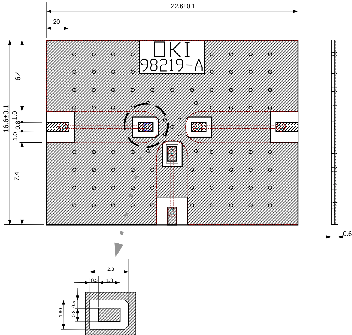
Test Board
