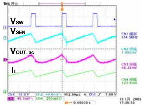
Fig 68. Switching waveform ( 12V_{IN} , 3.6V_{OUT} , R_{SEN}=0.27 )
