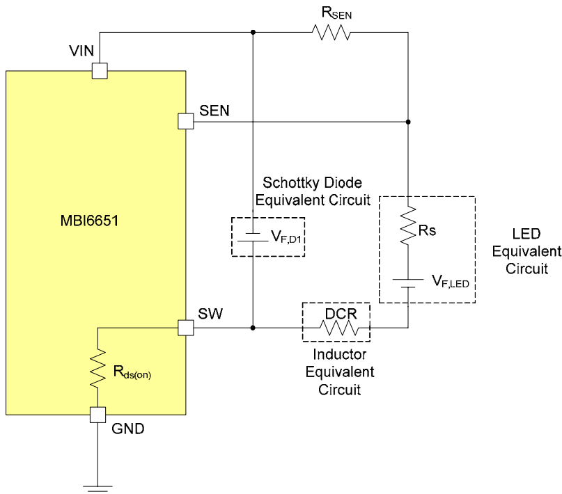
Fig. 78. The equivalent impedance in a MBI6651 application circuit
