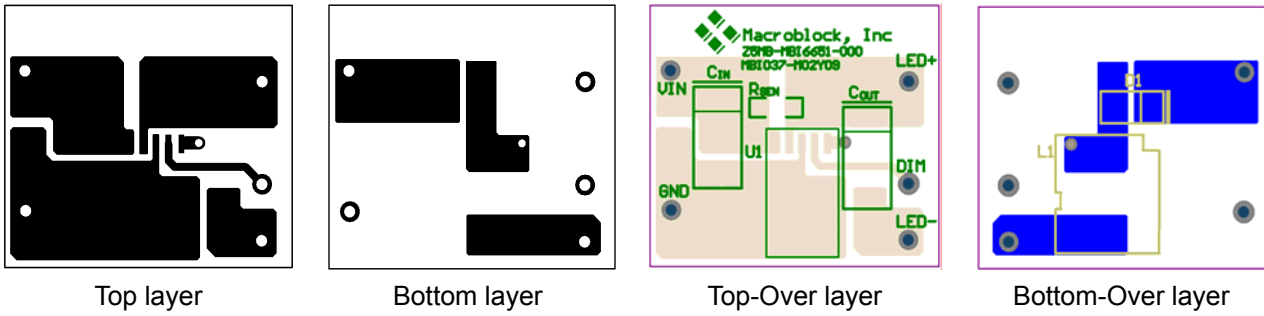
Fig. 86. The layout diagram of the MBI6651 GSD
