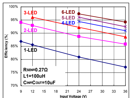
Fig 12. I_{OUT}=370mA
