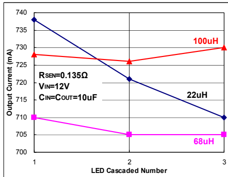
Fig 50. I_{OUT}=740mA
