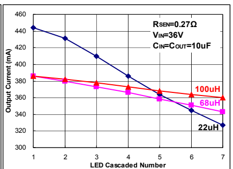
Fig 57. I_{OUT}=370mA
