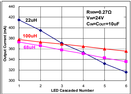
Fig 54. I_{OUT}=370mA
