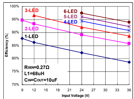
Fig 9. I_{OUT}=370mA
