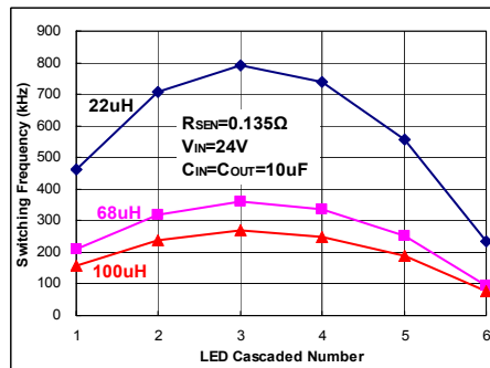
Fig 62. I_{OUT}=740mA
