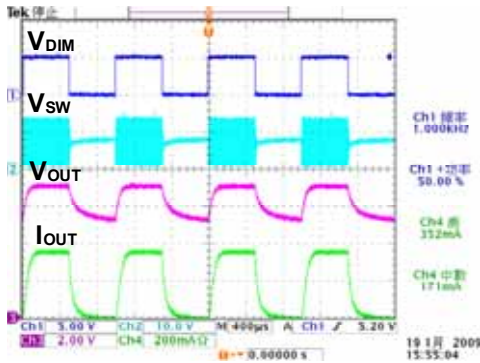
Fig 67. Dimming waveform ( V_{IN}=12V , R_{SEN}=0.27 , 2-LED)
