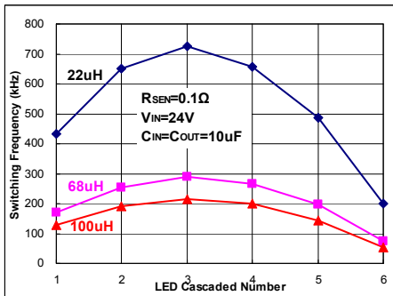
Fig 61. I_{OUT}=1A
