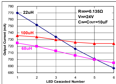
Fig 53. I_{OUT}=740mA
