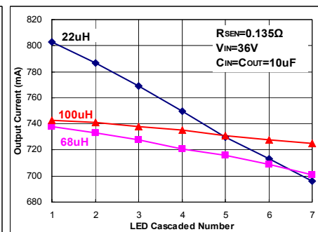
Fig 56. I_{OUT}=740mA
