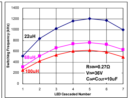
Fig 66. I_{OUT}=370mA
