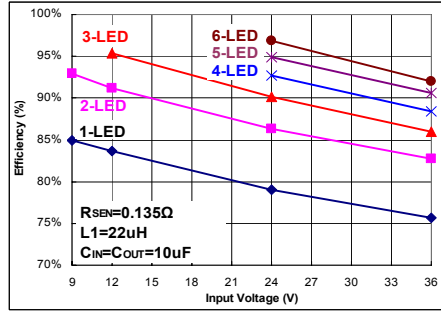
Fig 5. I_{OUT}=740mA
