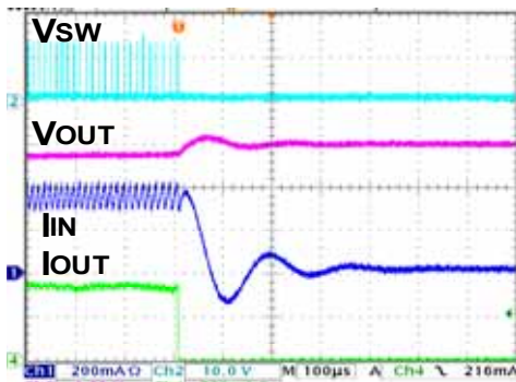
Fig. 82. Open-circuit protection
