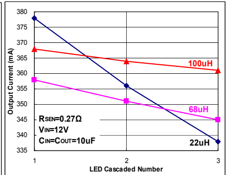
Fig 51. I_{OUT}=370mA
