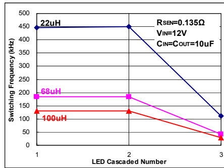
Fig 59. I_{OUT}=740mA
