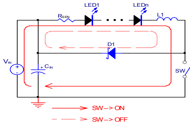
Fig. 85. Power loop of MBI6651
