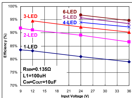
Fig 11. I_{OUT}=740mA
