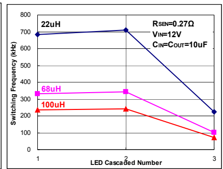
Fig 60. I_{OUT}=370mA
