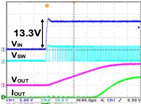
Fig 72. C IN =C OUT =Tantalum capacitor (10uF/50V)
