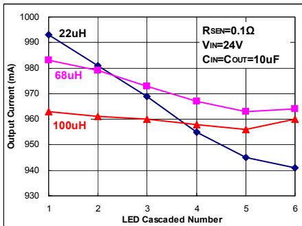
Fig 52. I_{OUT}=1A
