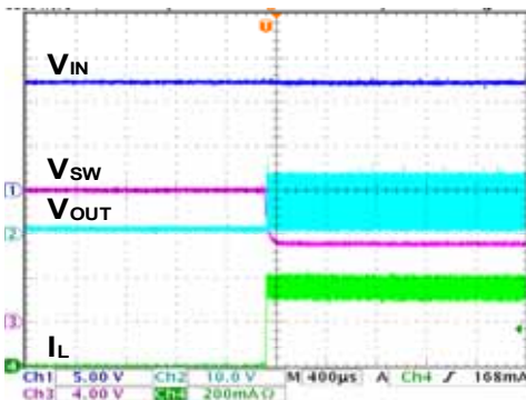
Fig 74. C IN =C OUT =Tantalum capacitor (10uF/50V)
