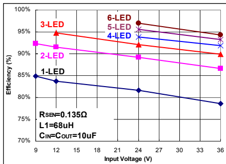
Fig 8. I_{OUT}=740mA
