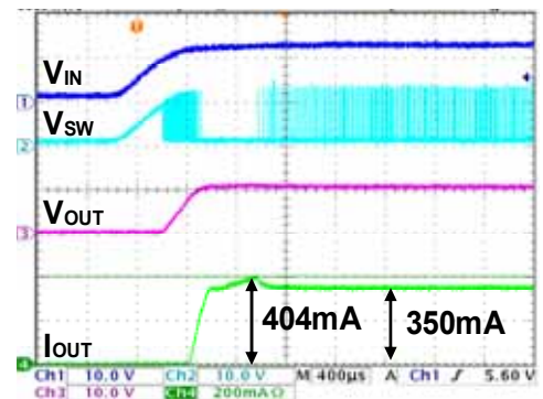
Fig. 79. The start-up waveform @ V_{IN}=12V, V_{OUT}= 10.8, R_{SEN}=0.27
