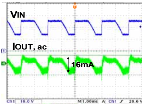
Fig 71. L1=100\mu H
