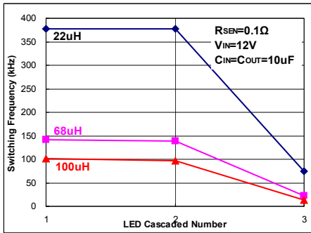
Fig 58. I_{OUT}=1A
