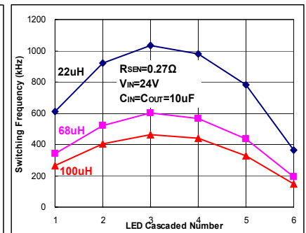
Fig 63. I_{OUT}=370mA
