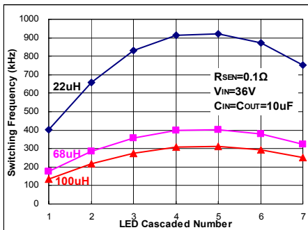
Fig 64. I_{OUT}=1A
