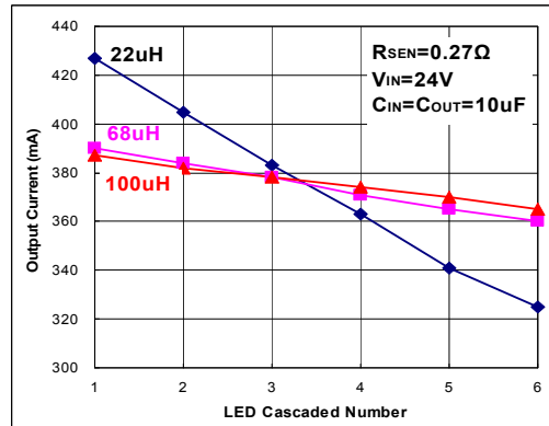
Fig 37. I OUT =370 mA
