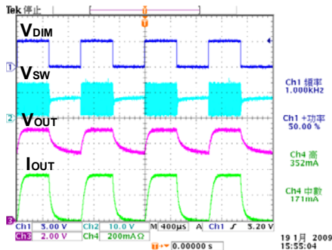
Fig 46. Dimming waveform ( V_{IN}=12V , R_{SEN}=0.27\Omega , 2-LED)
