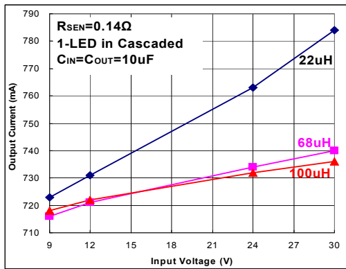
Fig 22. I_{OUT}=715 mA
