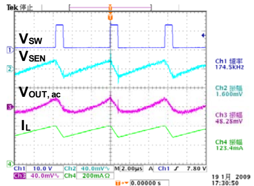
Fig 47. Switching waveform ( 12V_{IN} , 3.6V_{OUT} , R_{SEN}=0.27\Omega )
