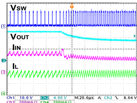
Figure 62. Short-circuit protection
