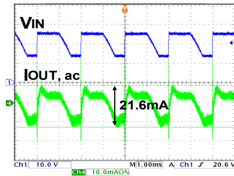
Fig49. L1=68\mu H
