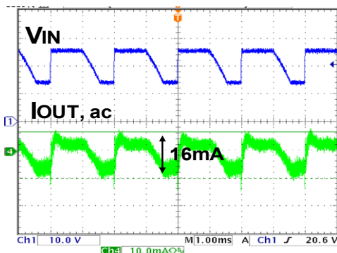
Fig 50. L1=100\mu H
