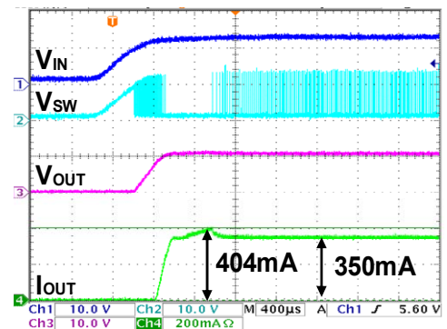
Figure 58. The start-up waveform @ V_{IN}=12V , V_{OUT}= 10.8 , R_{SEN}=0.27\Omega
