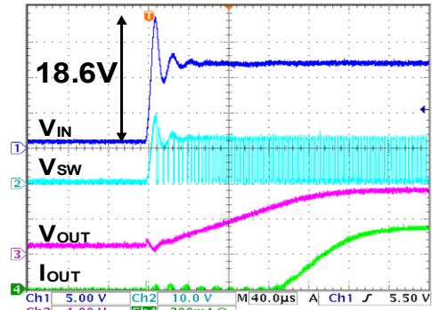
Fig 52. C_{IN}=C_{OUT} =Ceramic capacitor (2 x 4.7uF/35V)
