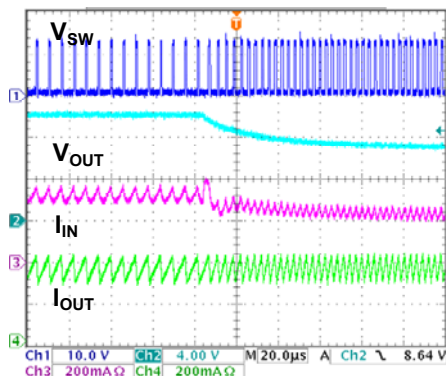
Fig. 72 Short-circuited protection
