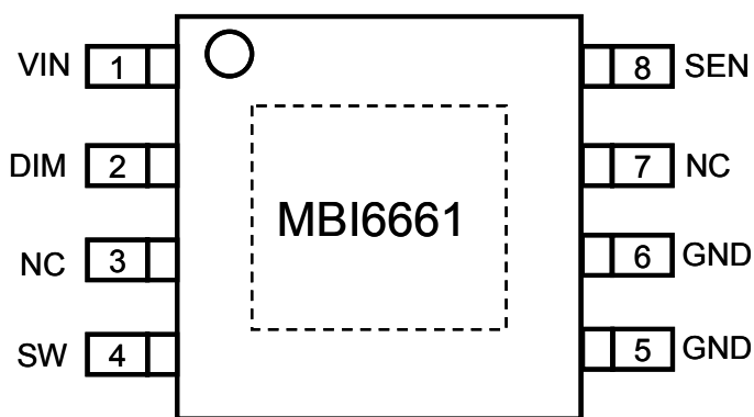
MBI6661GD
