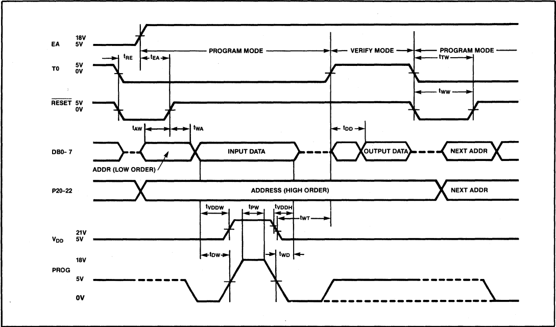
Timing Diagram for Programming/Verify Mode:
