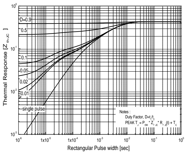
Fig.29 IGBT Transient Thermal Impedance
