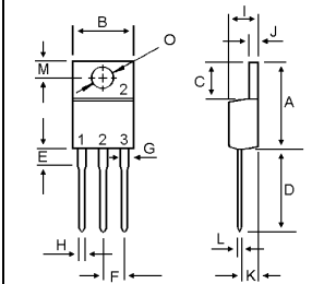
TO-220AB
