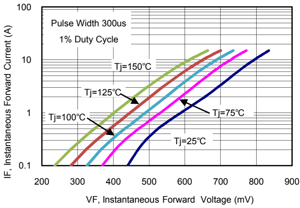
Figure 5: Typical Forward Characteristics (MBR10U150CT) (Per Leg)
