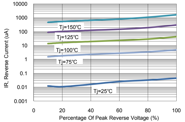
Figure 8: Typical Reverse Characteristics (MBR10U200CT) (Per Leg)
