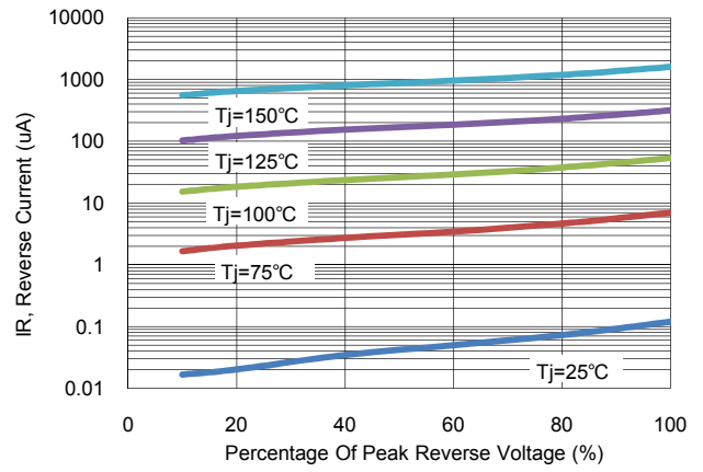
Figure 6: Typical Reverse Characteristics (MBR10U150CT) (Per Leg)
