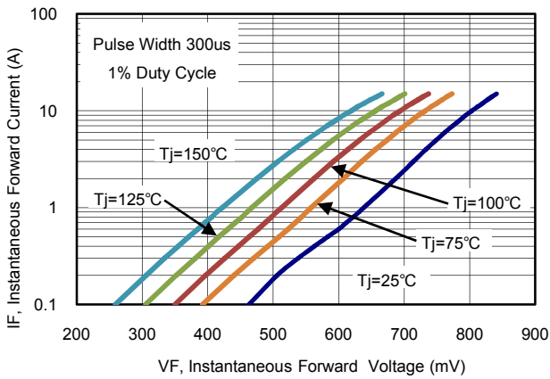
Figure 7: Typical Forward Characteristics (MBR10U200CT) (Per Leg)
