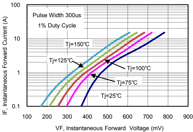
Figure 3: Typical Forward Characteristics (MBR10U100CT) (Per Leg)
