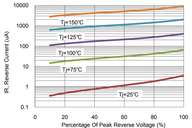
Figure 4: Typical Reverse Characteristics (MBR10U100CT) (Per Leg)
