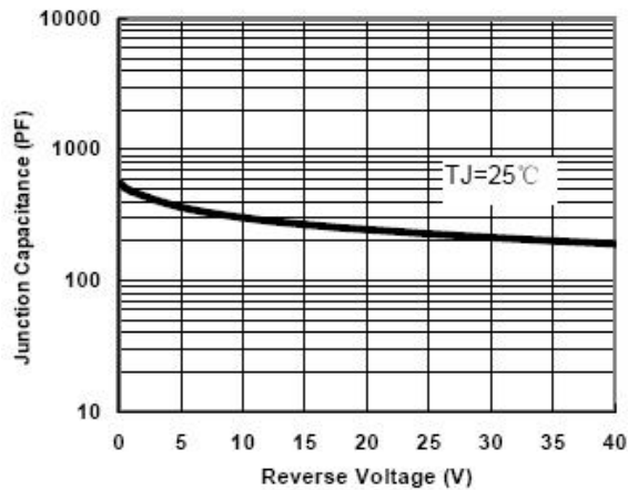
Fig.1-Typical Junction Capacitance
