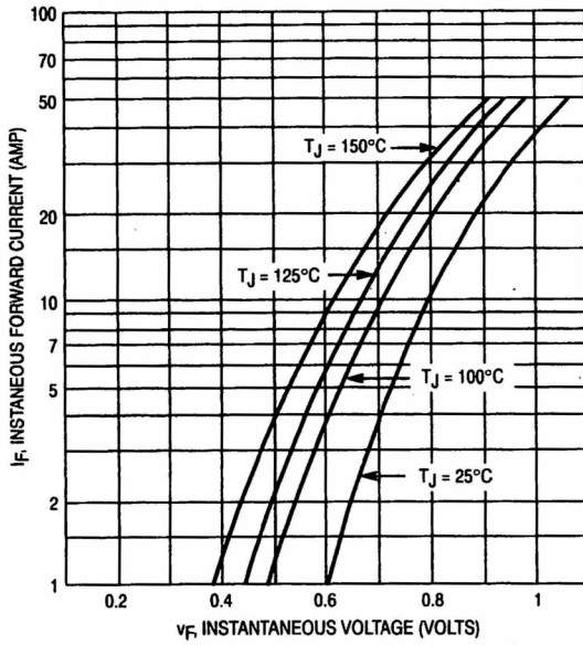
Figure 1. Typical Forward Voltage (Per Leg)
