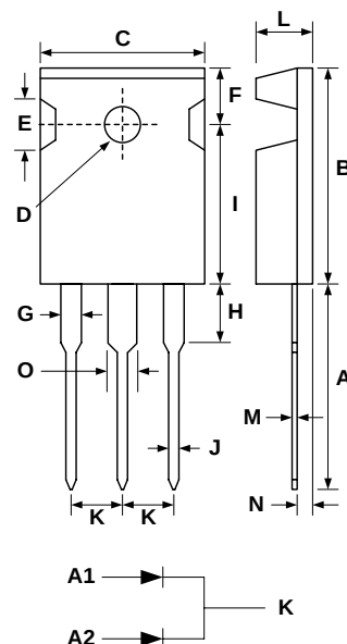
TO-247AD
