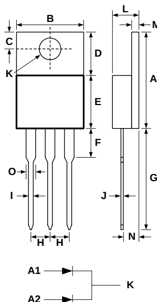
TO-220AB
