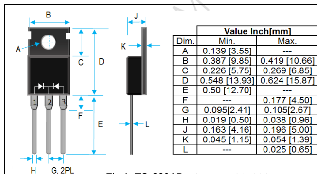
Fig 1. TO-220AB FOR MBR30L60CT
