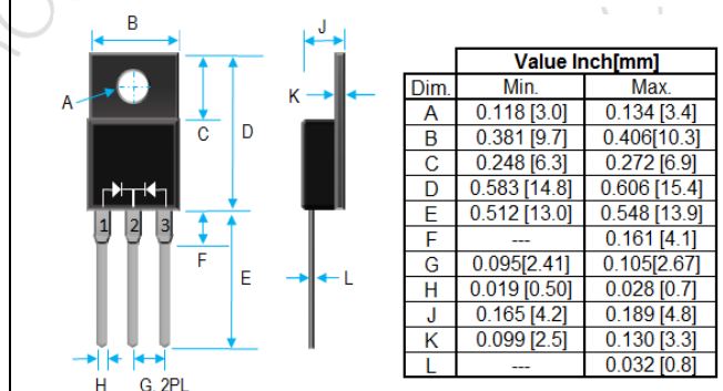
Fig 2. ITO-220AB FOR MBR30L60FCT
