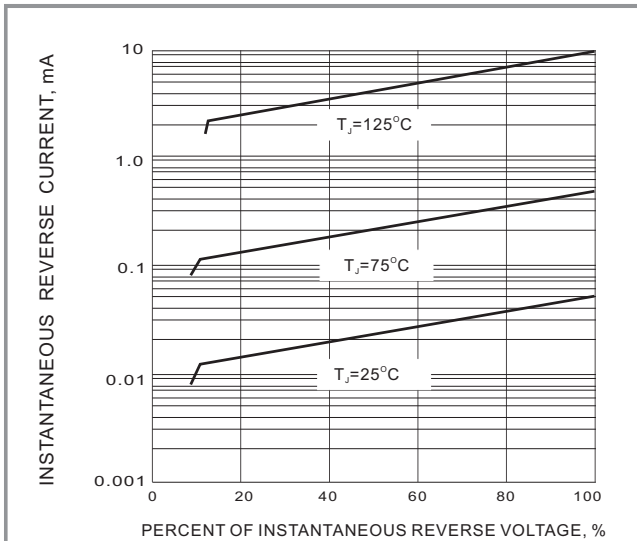
Fig. 3-TYPICAL REVERSE CHARACTERISTIC
