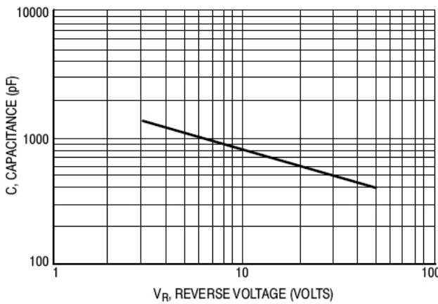
Figure 3. Typical Capacitance Per Leg
