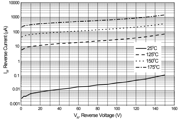
Figure 2. Typical Reverse Characteristics
