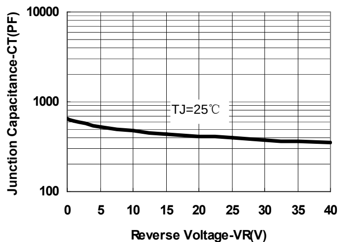
Fig.1-Typical Junction Capacitance
