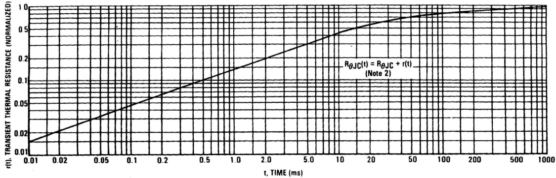
FIGURE 8 — THERMAL RESPONSE
