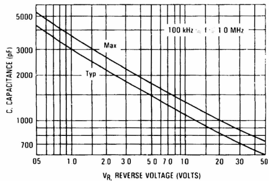
FIGURE 4 — CAPACITANCE
