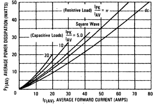
FIGURE 6 — POWER DISSIPATION
