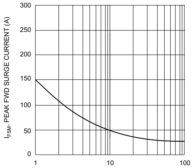
Fig. 4 Max Non-Repetitive Surge Current
