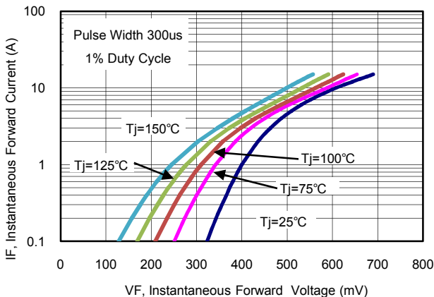
Figure 5: Typical Forward Characteristics (MBRB3060CT) (Per Leg)
