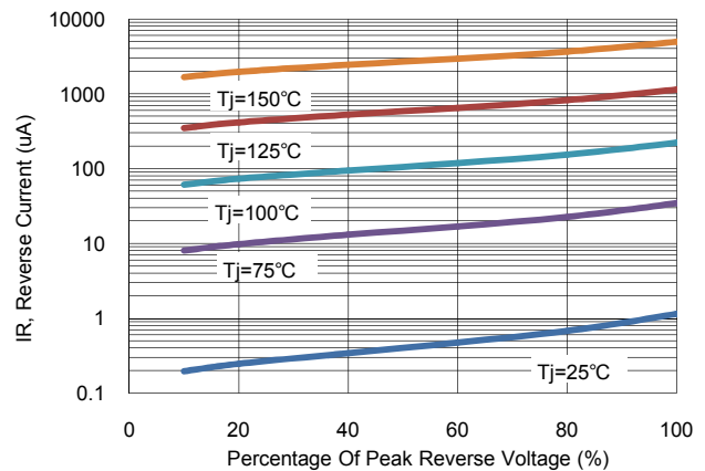
Figure 4: Typical Reverse Characteristics (MBRB3040CT) (Per Leg)
