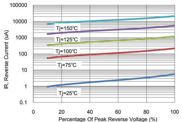
Figure 6: Typical Reverse Characteristics (MBRB3060CT) (Per Leg)
