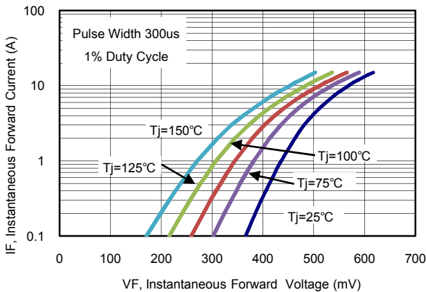
Figure 3: Typical Forward Characteristics (MBRB3040CT) (Per Leg)
