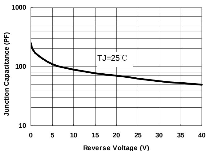
Fig.1-Typical Junction Capacitance
