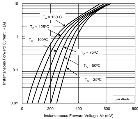
Fig. 1 - Forward Characteristics
