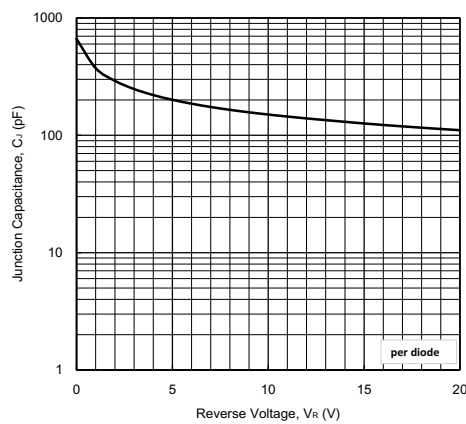
Fig. 5 - Junction Capacitance
