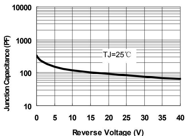
Fig.1-Typical Junction Capacitance
