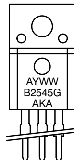
ISOLATED TO-220 CASE 221D STYLE 3
