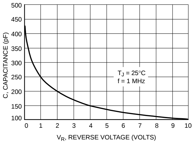
Figure 6. Typical Capacitance
