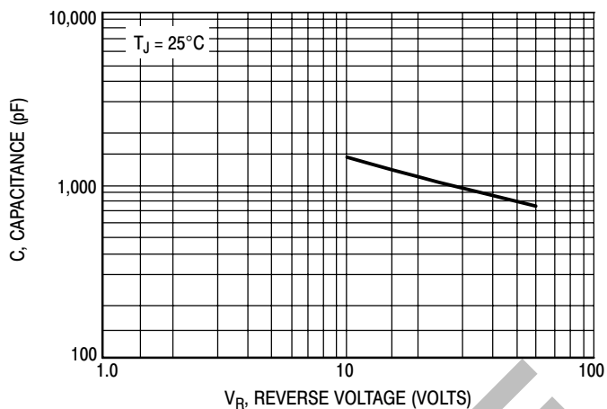
Figure 7. Capacitance
