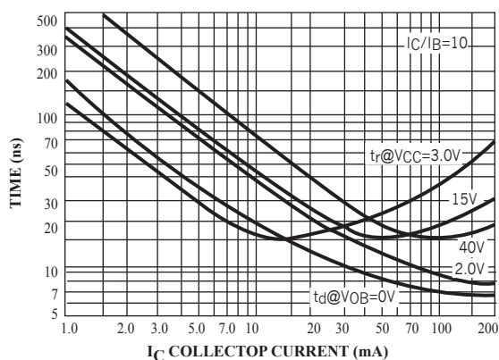
Figure 23. Turn-On Time
