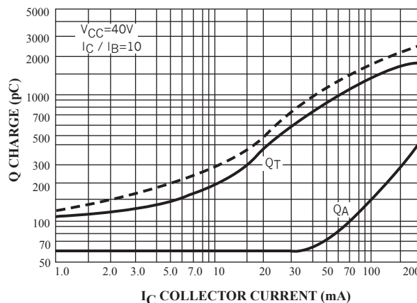
Figure 4. Charge Data
