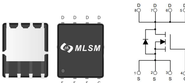
PDFN5X6-8L view
