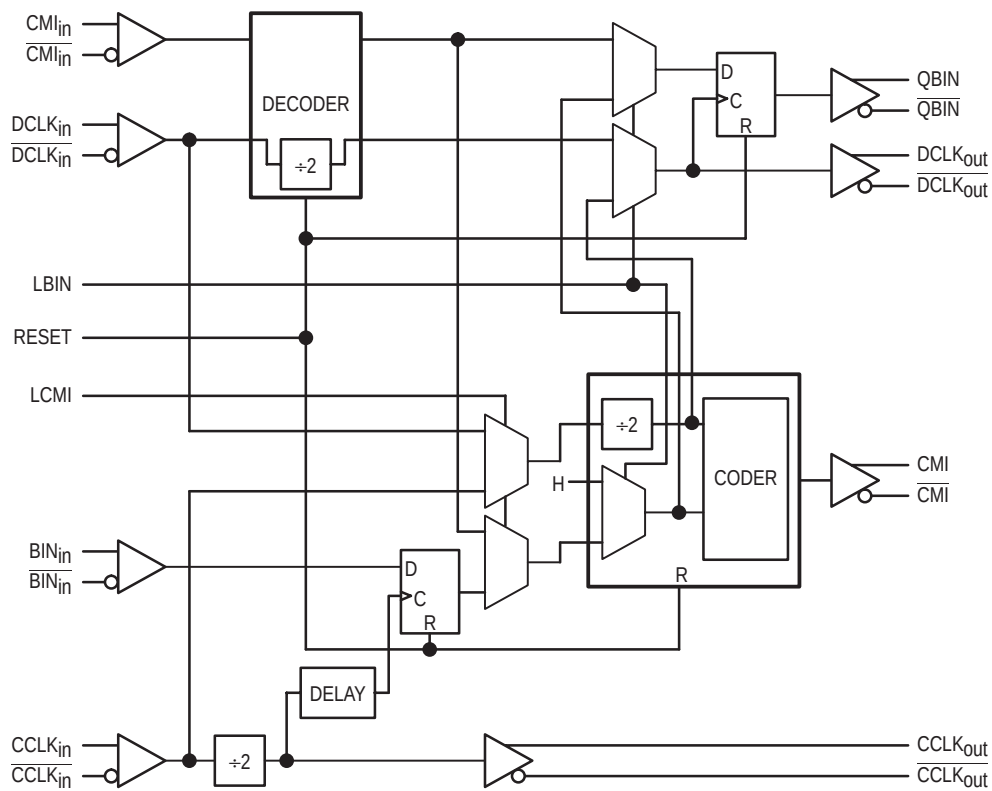
BLOCK DIAGRAM
