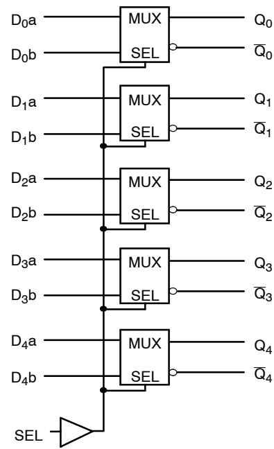
Figure 2. Logic Diagram
