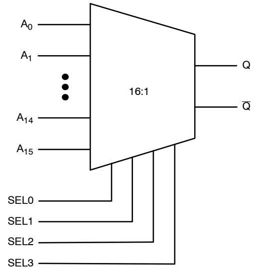
Figure 2. Logic Diagram
