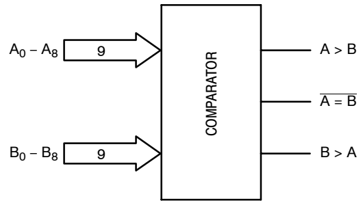
Figure 2. Logic Diagram
