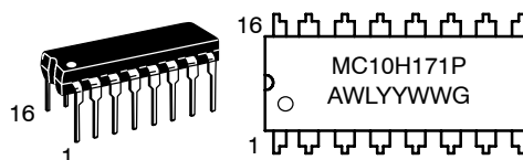
PDIP-16 P SUFFIX CASE 648
