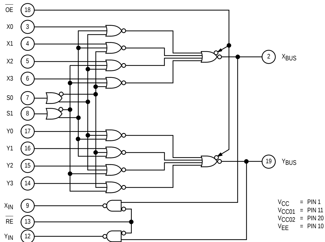
LOGIC DIAGRAM
