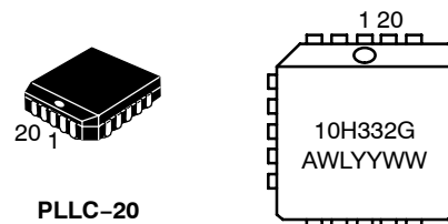
PLLC-20 FN SUFFIX CASE 775
