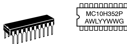
PDIP-20 P SUFFIX CASE 738
