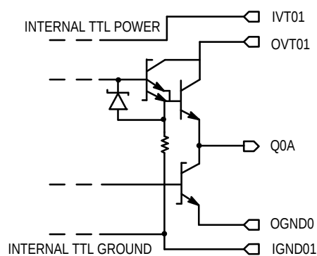
Figure 1. Output Structure
