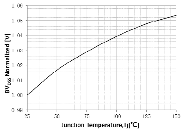
Breakdown Voltage Variation vs T_j
