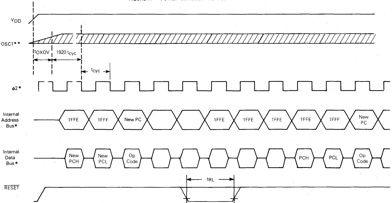
FIGURE 11 – POWER-ON RESET AND \overline{RESET}
