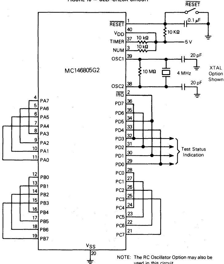
FIGURE 16 — SELF-CHECK CIRCUIT
