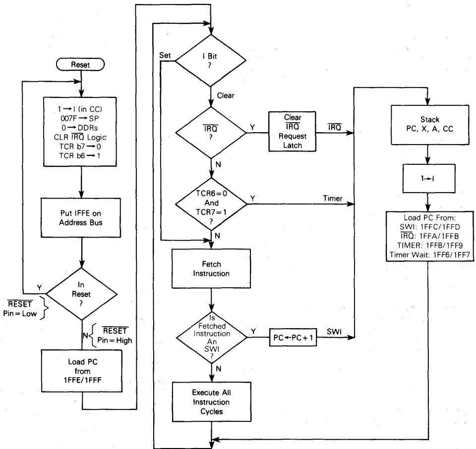
FIGURE 20 — RESET AND INTERRUPT PROCESSING FLOWCHART
