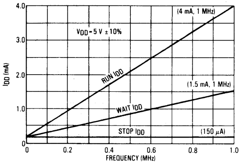
FIGURE 4 – MAXIMUM I_{DD} vs FREQUENCY
