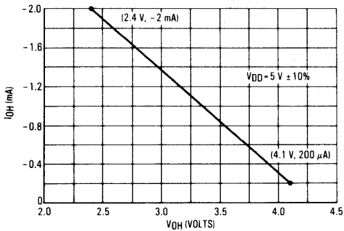
FIGURE 8 – MINIMUM I_{OH} , PORT A AND B
