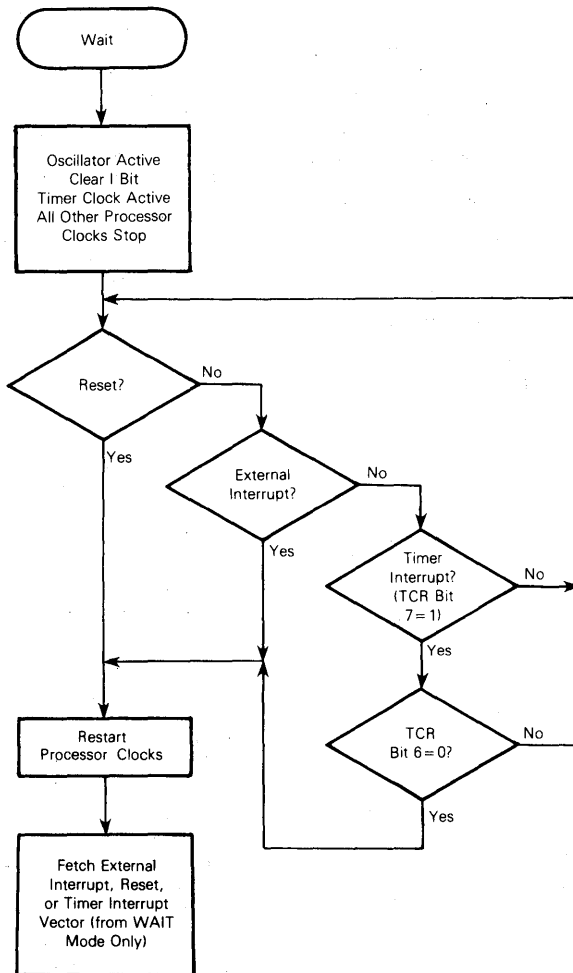
FIGURE 23 — WAIT FUNCTION FLOWCHART
