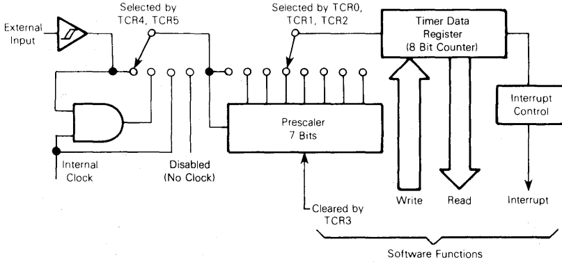
FIGURE 24 — TIMER BLOCK DIAGRAM
