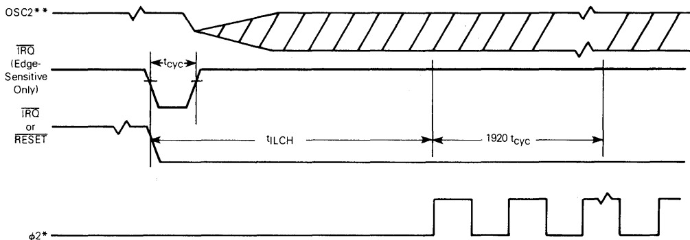
FIGURE 12 — STOP RECOVERY AND POWER-ON RESET
