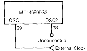
(e) External Clock Source Connections
