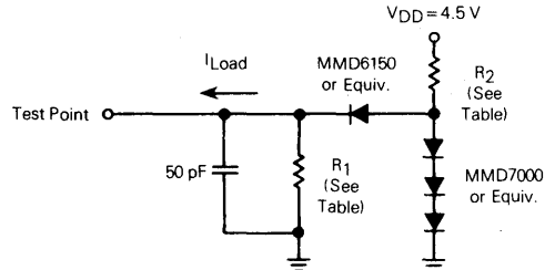
FIGURE 2 — EQUIVALENT TEST LOAD
