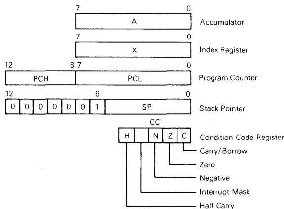
FIGURE 18 — PROGRAMMING MODEL
