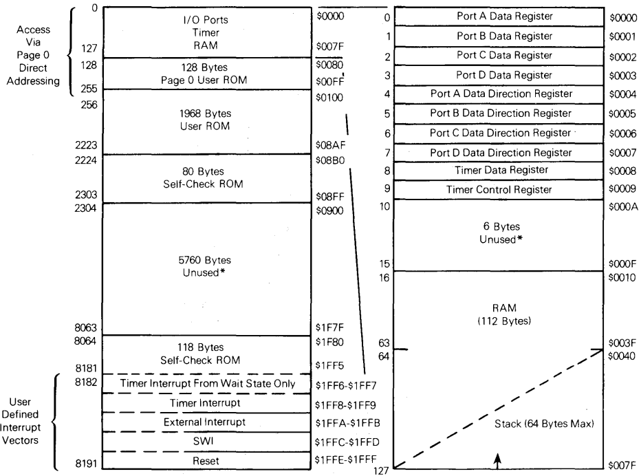
FIGURE 17 — ADDRESS MAP
